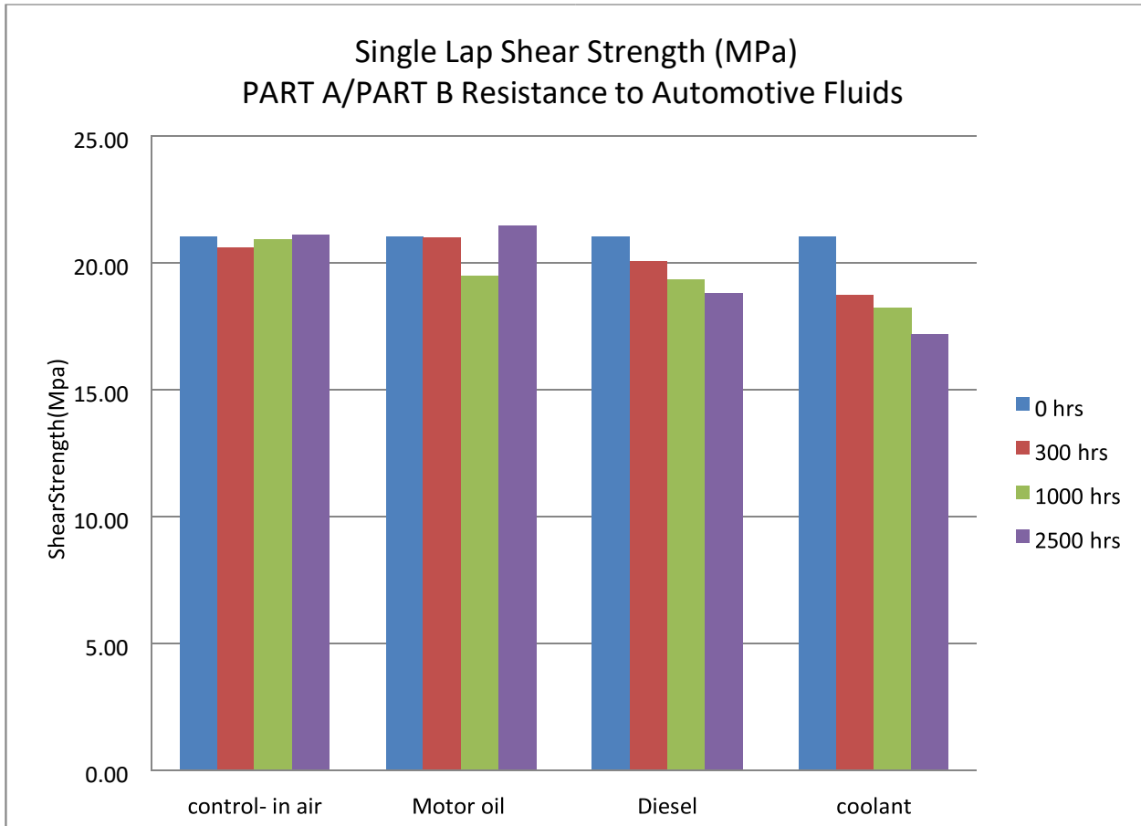
Single Lap Shear Strength in MPa (Tests conducted at 24 C, 50% RH (ASTM D1002))
