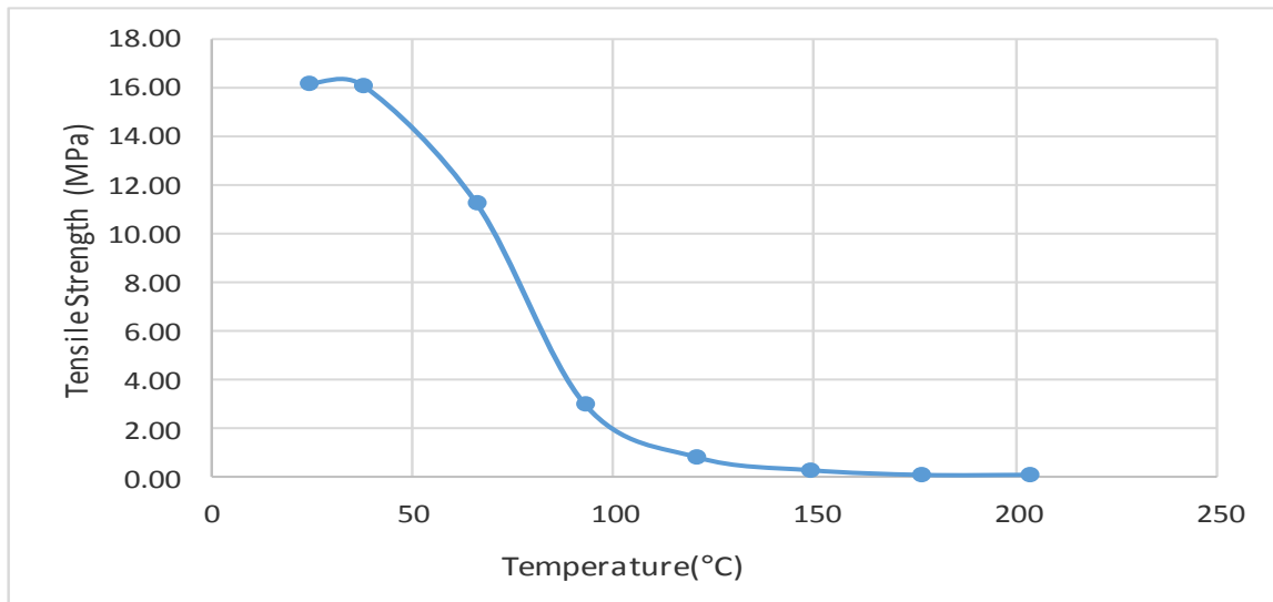
Figure 1: SG300-15 Shear Strength versus Temperature
